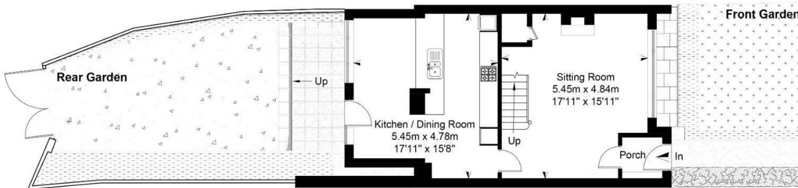
Ground Floor
